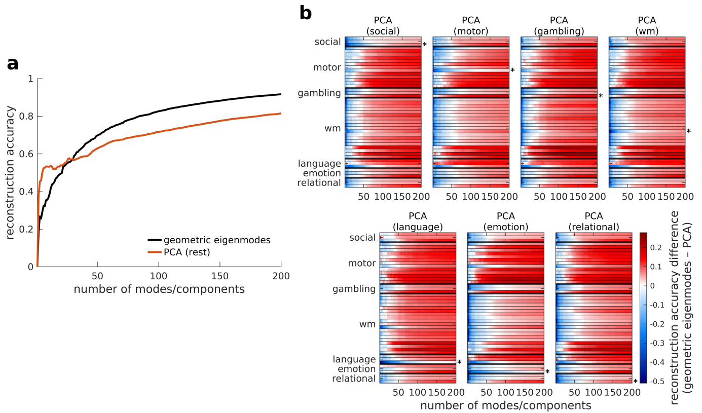
Extended Data Fig. 4 | Reconstruction accuracy achieved by geometric eigenmodes and PCA. (a) Reconstruction accuracy of resting-state FC. (b) Comparison of the reconstruction accuracy of all 47 HCP task-contrast maps, which have been grouped here by broad types (Supplementary
